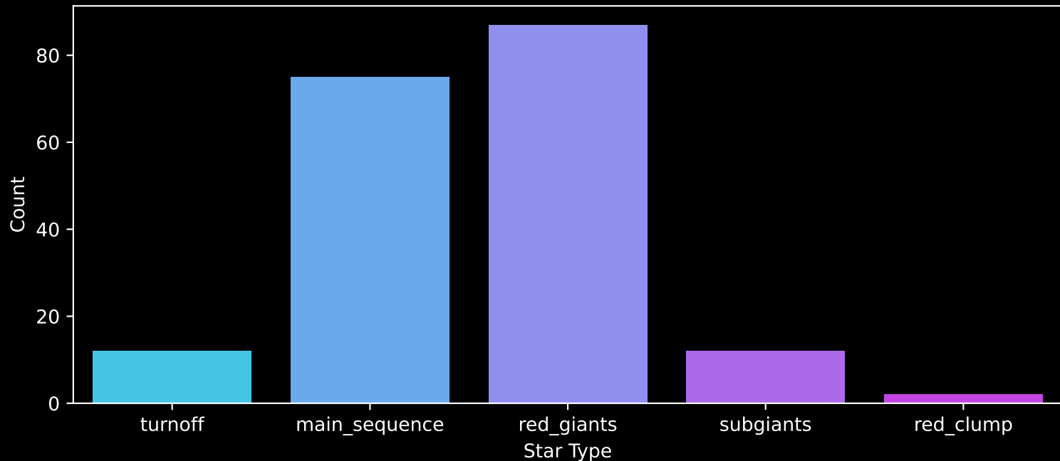
APOGEE DR17 Field: [K2_C6_327+45_btx] Count plot of Star Type
