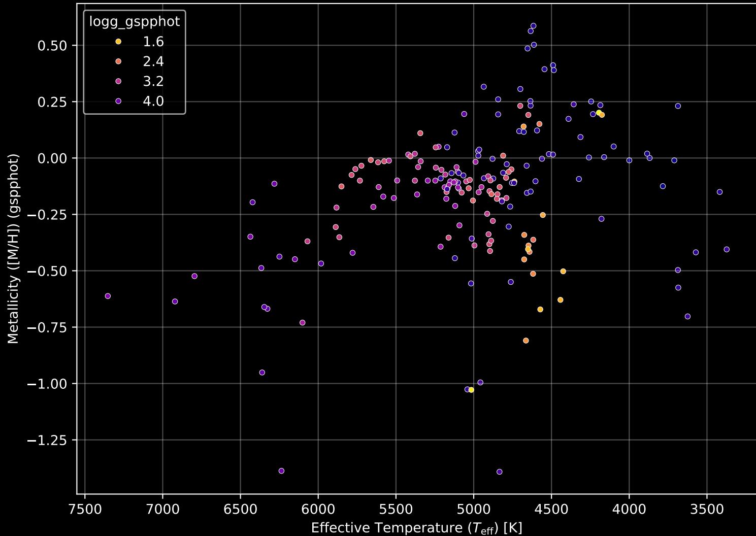
APOGEE DR17 Field: [K2_C6_327+45_btx] Stellar Population Parameters (n= 188)
