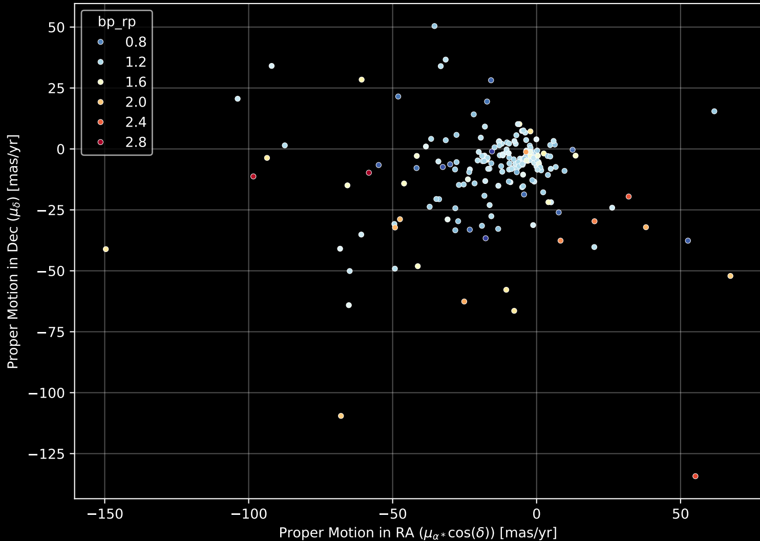
APOGEE DR17 Field: [K2_C6_327+45_btx] Proper Motion Diagram (n= 188)
