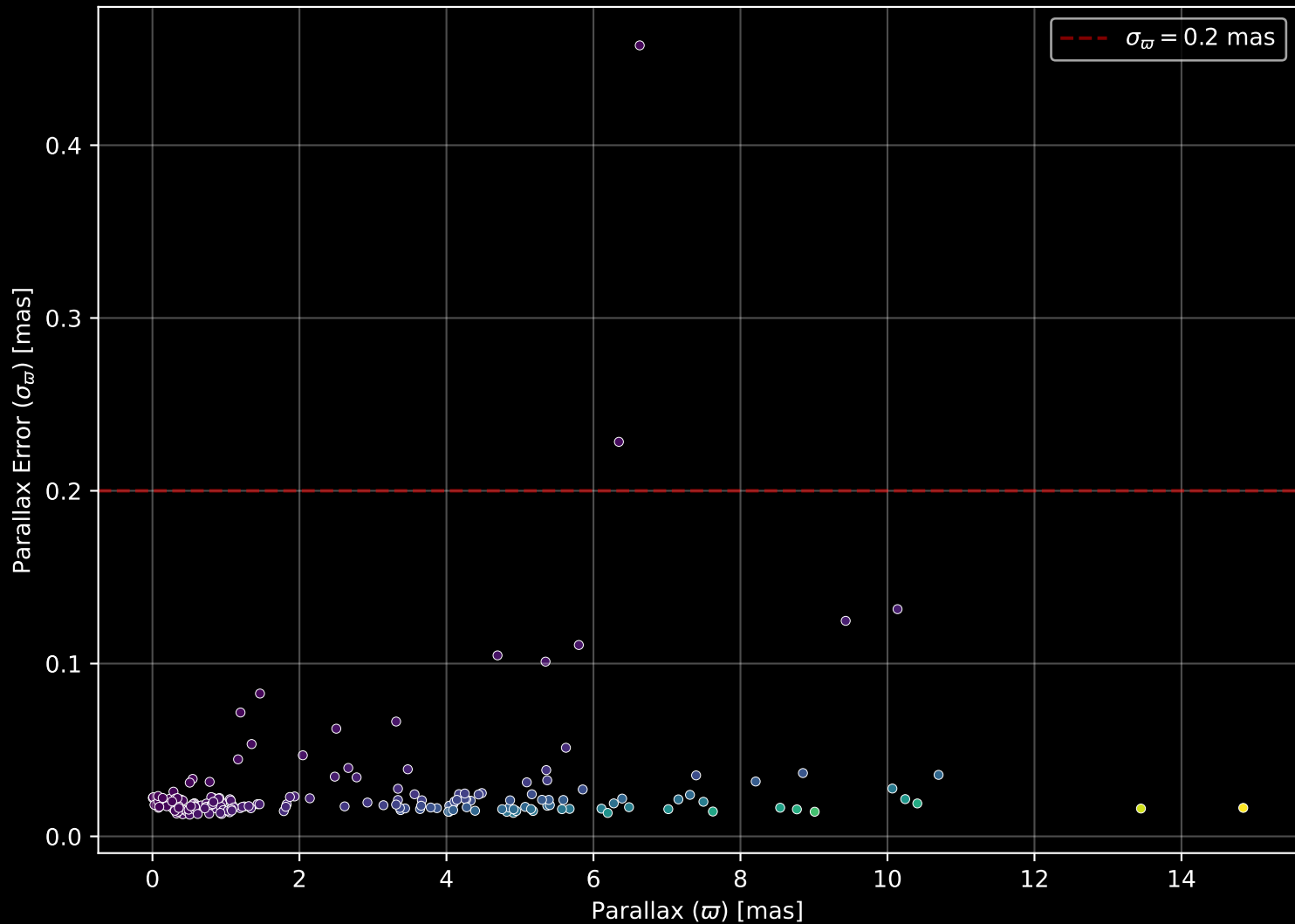
APOGEE DR17 Field: [K2_C6_327+45_btx] Parallax Quality (n= 188)
