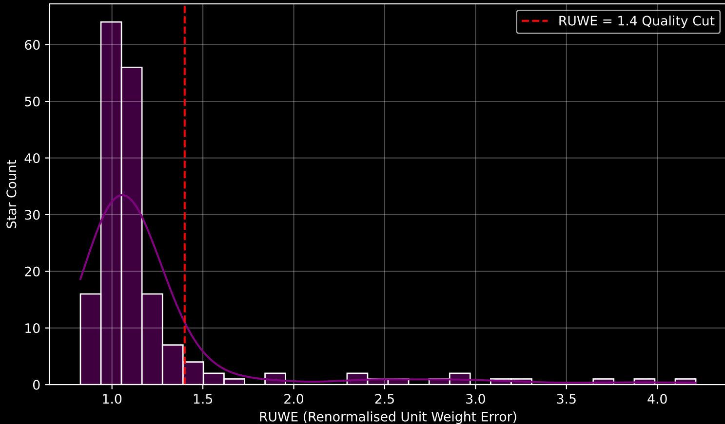
GAPOGEE DR17 Field [K2_C6_327+45_btx] RUWE Distribution (n= 180)
