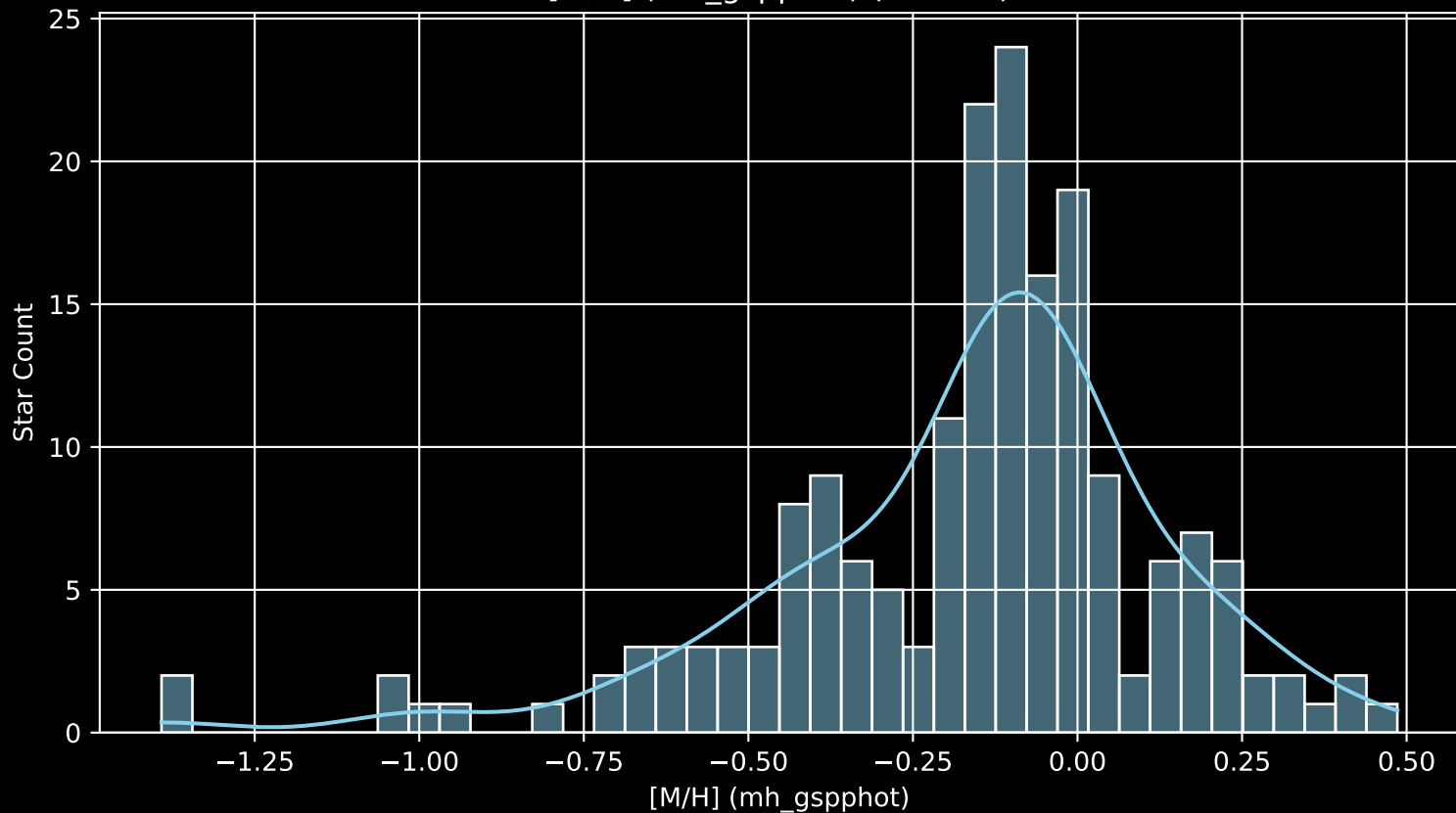
APOGEE DR17 Field: [K2_C6_327+45_btx [M/H] (mh_gspphot) (n= 185)
